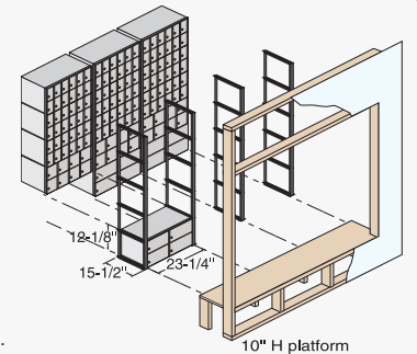
Individual rack ladder mailbox with optional hinged locking rear cover (#2252) displayed
